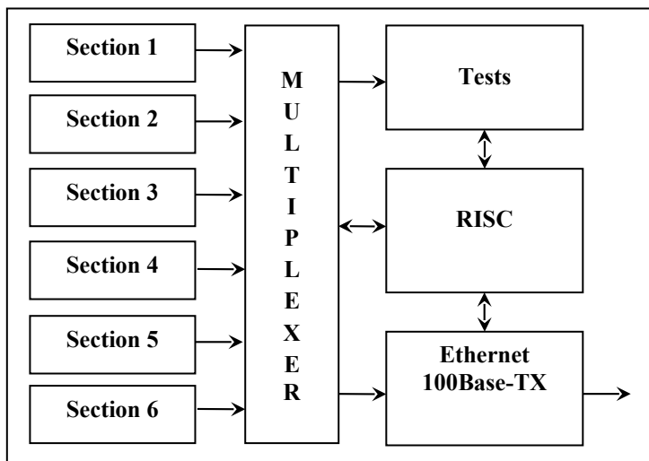
Fig. 3. Outline of 100Mbit/s random generator
